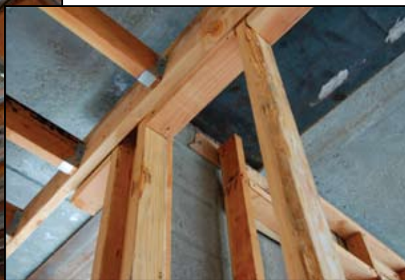
Interior non-structural wall connections.
